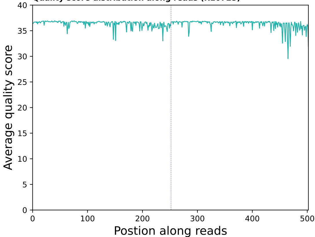
Quality score distribution along reads (R10725)
